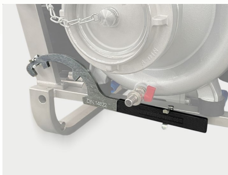
Fixing for coupling wrench Storz acc. DIN 14822-2
