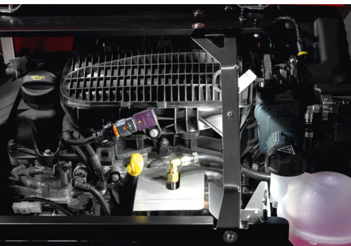
Water-cooled gasoline engine, silent engine operation with low vibration, exhaust gas cooling system and illuminated maintenance access
