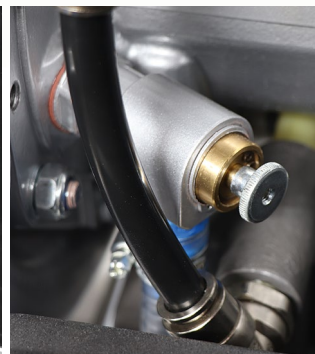
Mechanical thermostatic valve with flushing function as standard
